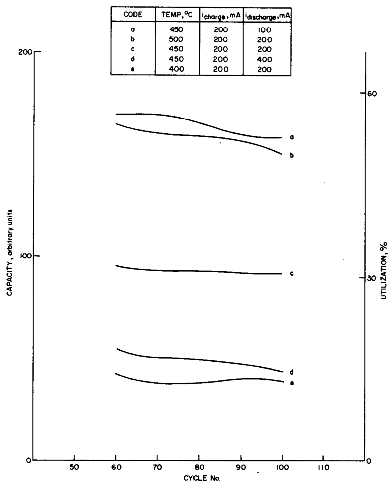
Fig. 4. The effect of operating temperature and discharge current on the capacity of pelletized LiAl-FeS cells.
