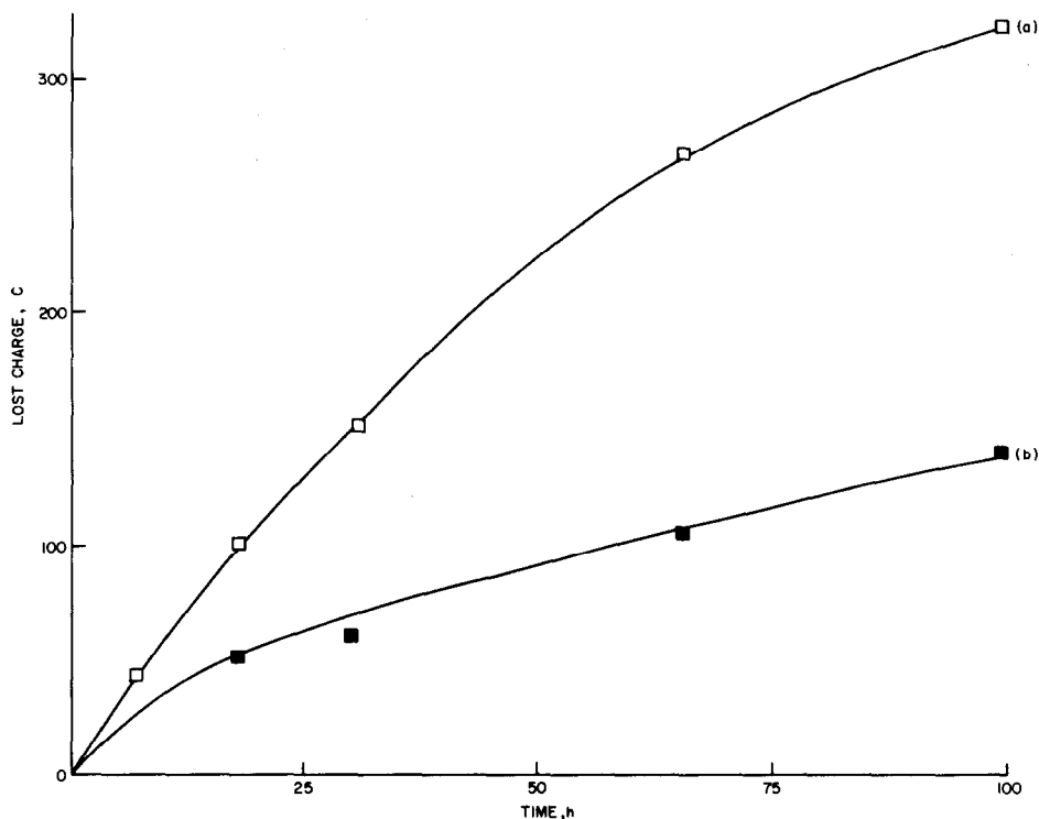
Fig. 7. Rate of charge loss for cells left on open-circuit at full charge ( T = 450^{\circ}\text{C} ). (a) After 2000 cycles ( \sim 30 weeks on test); (b) after 200 cycles ( \sim 3 weeks on test).
