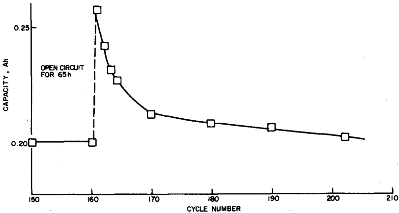
Fig. 6. Capacity enhancement effect exhibited by pelletized cells following a period of 65 h on open-circuit in the fully discharged condition.
